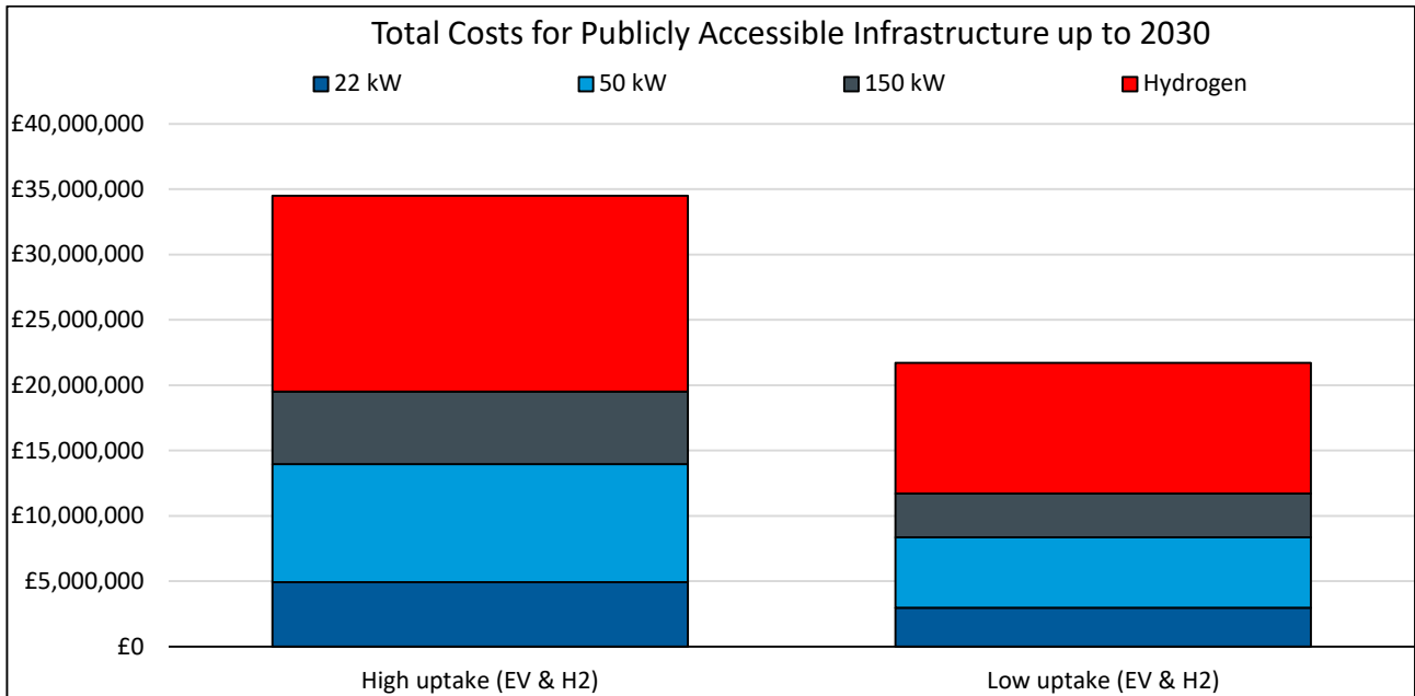
Figure 12-17 - Total public infrastructure costs up to 2030, Peninsula Transport
