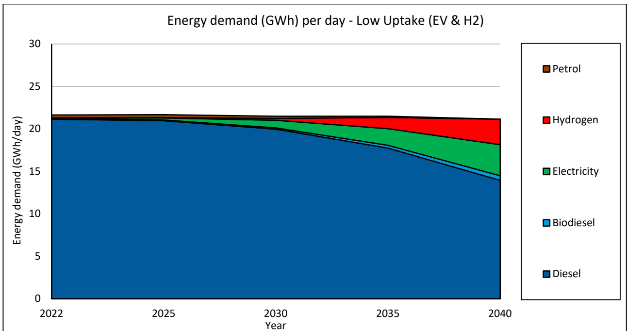
Figure 12-16 - Electric vehicle & Hydrogen only scenario - Low uptake, total energy demand per day for all LGVs and HGVs, Peninsula Transport
