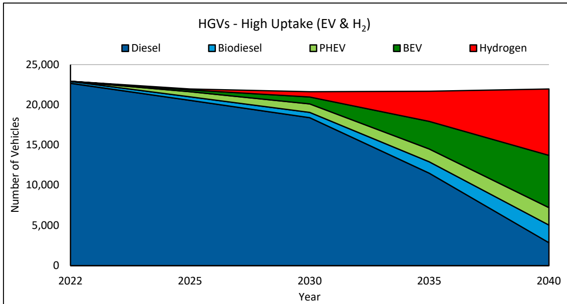
Figure 12-3 - Electric vehicles & Hydrogen only scenario HGVs - High uptake, Western Gateway
