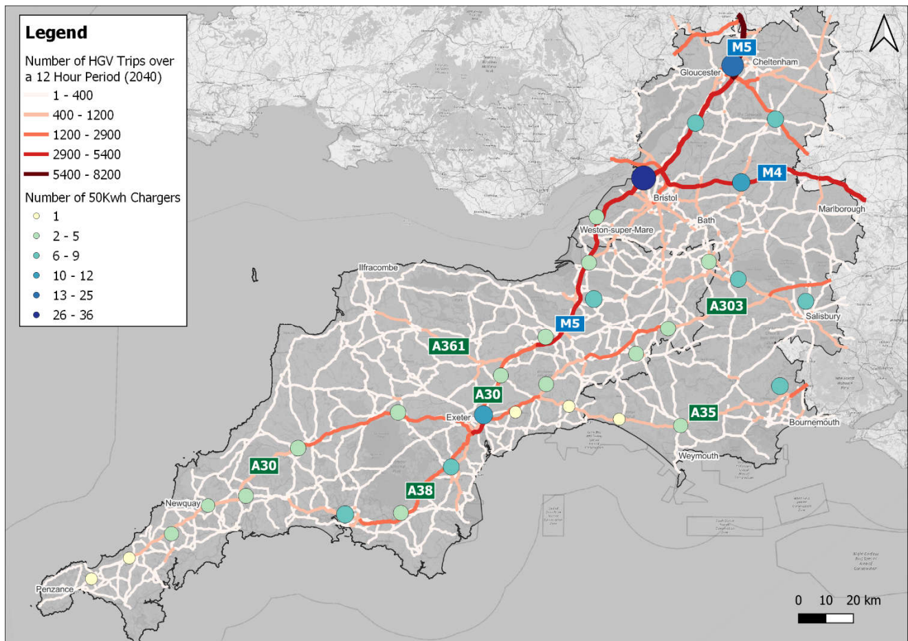
Figure 15-5 - Potential distribution of 50Kwh charging facilities
