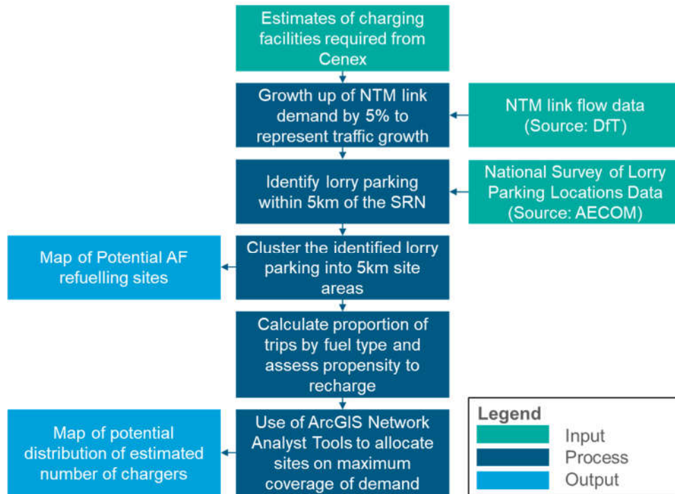
Figure 15-1 - Methodology for allocating charging facilities
