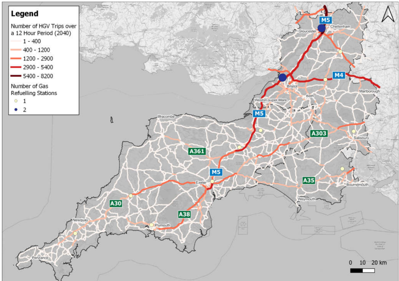
Figure 15-9 - Potential distribution of gas refuelling facilities
