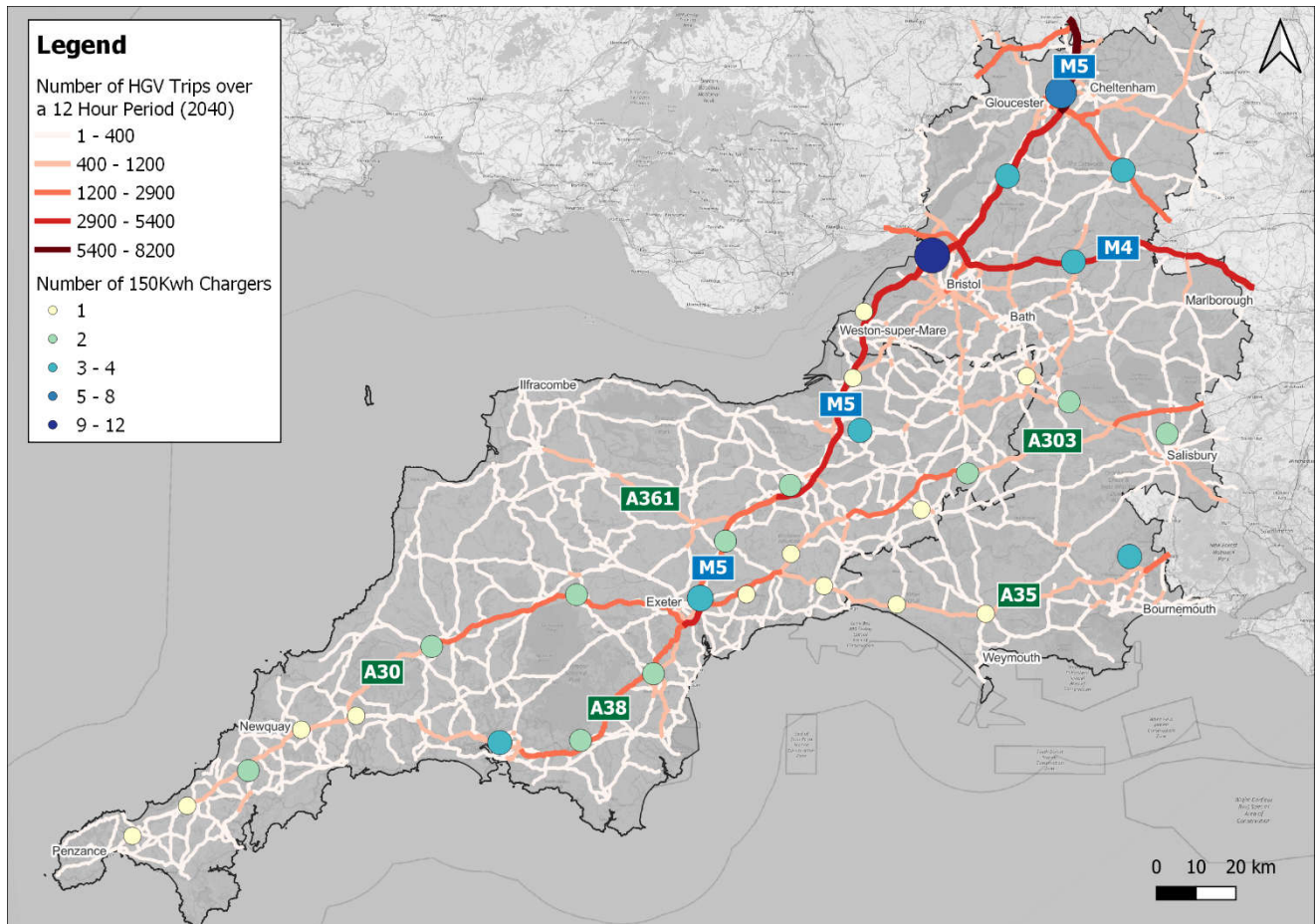
Figure 15-6 - Potential distribution of 150Kwh charging facilities
