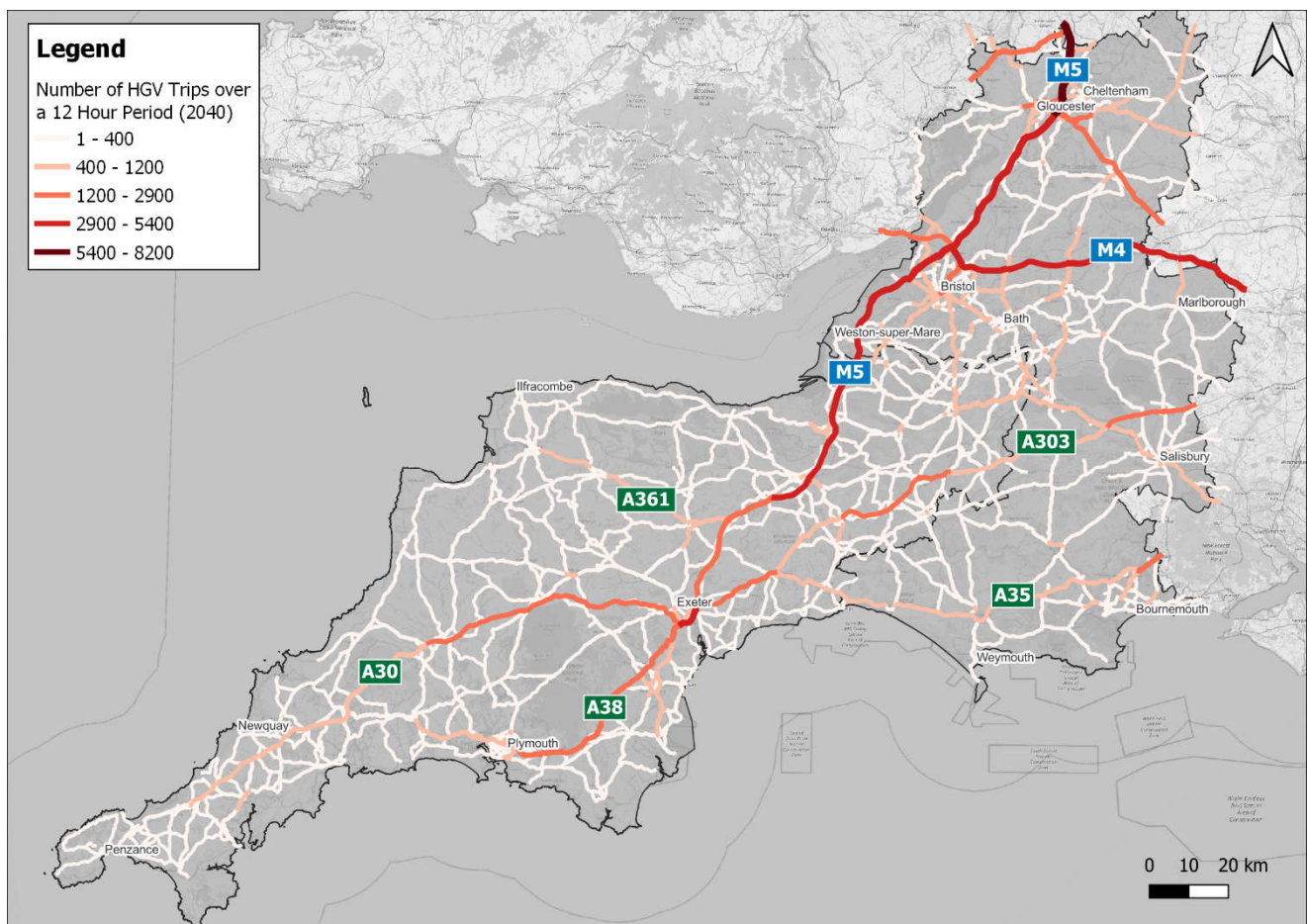
Figure 15-2 - Estimated 12-hour HGV flows in 2040
