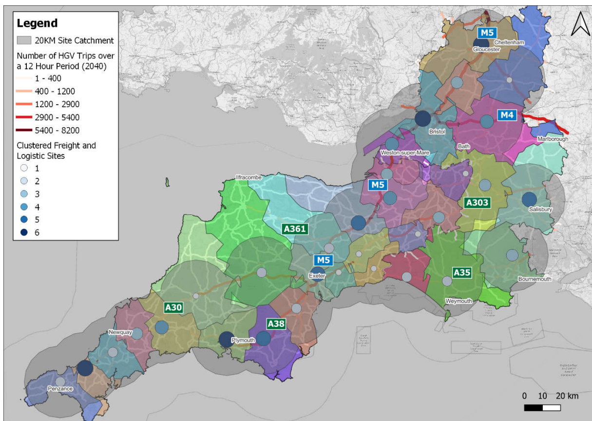
Figure 15-7 - Approximate catchment of freight clusters used for electric vehicle recharging based on demand allocation alongside the recommended 20-kilometre catchment areas
