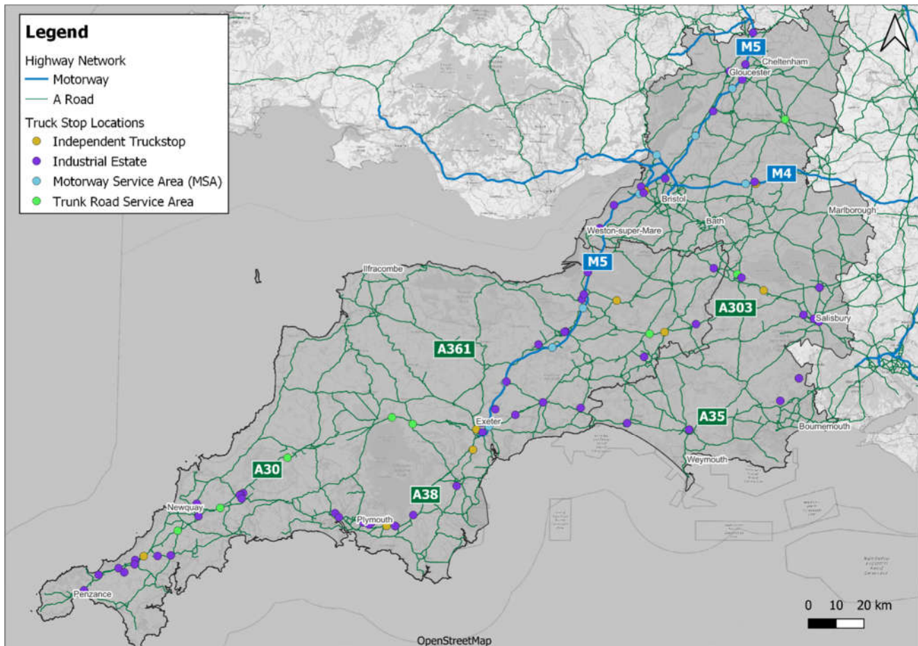
Figure 15-3 - Location of current freight and logistics sites which could potentially house charging infrastructure
