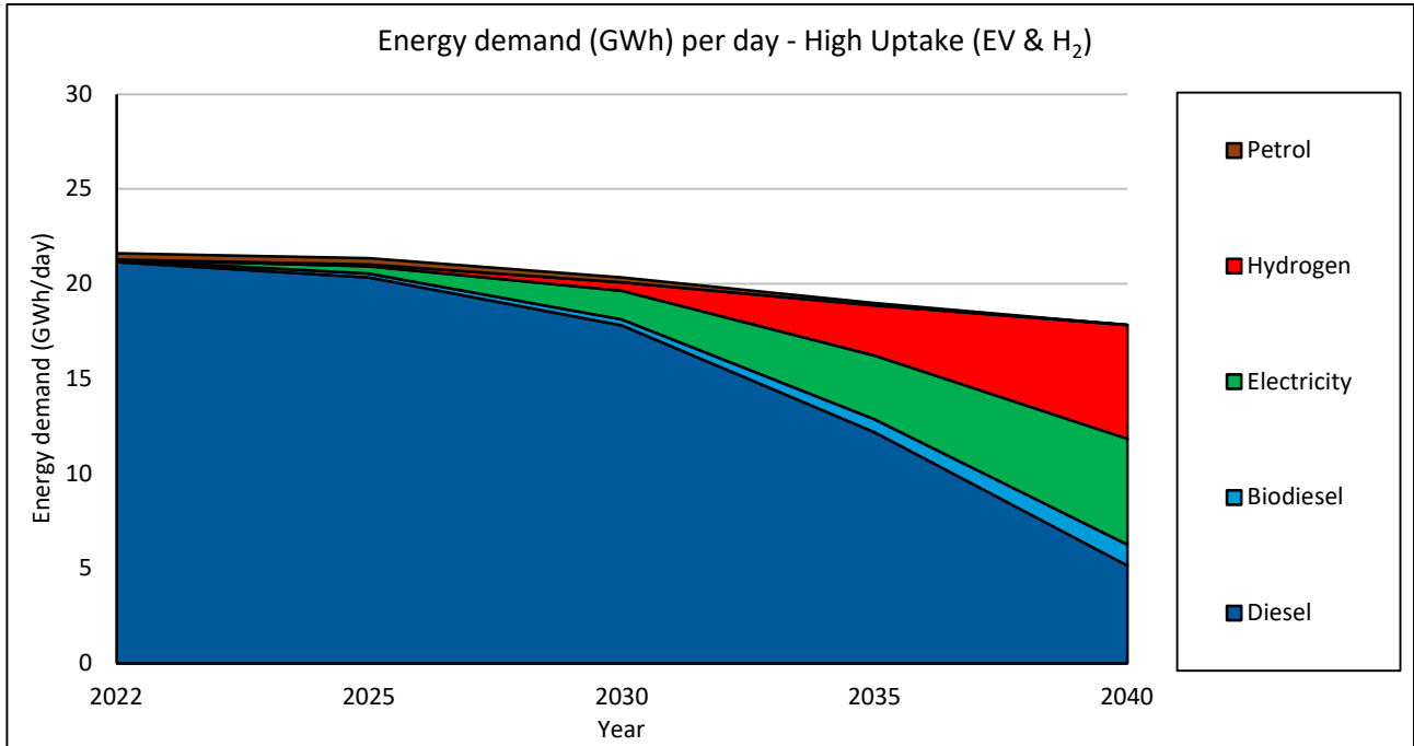
Figure 12-15 - Electric vehicle & Hydrogen only scenario - High uptake, total energy demand per day for all LGVs and HGVs, Peninsula Transport
