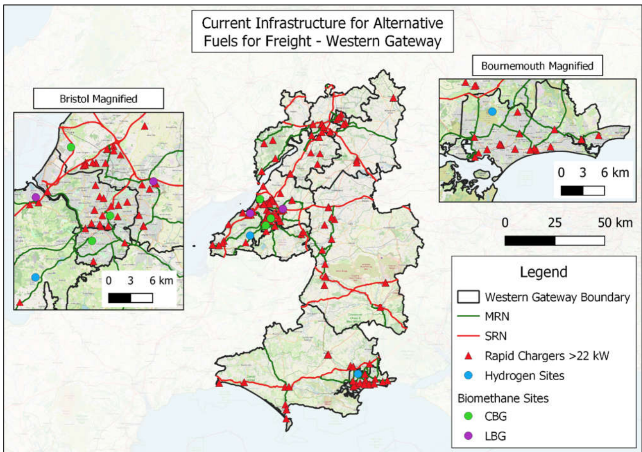
Figure 12-1 - Current infrastructure for alternative fuels for freight - Western Gateway
