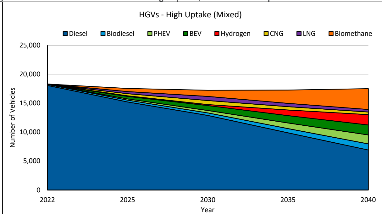
Figure B-3 - Mixed fuel scenario HGVs - High uptake, Peninsula Transport
