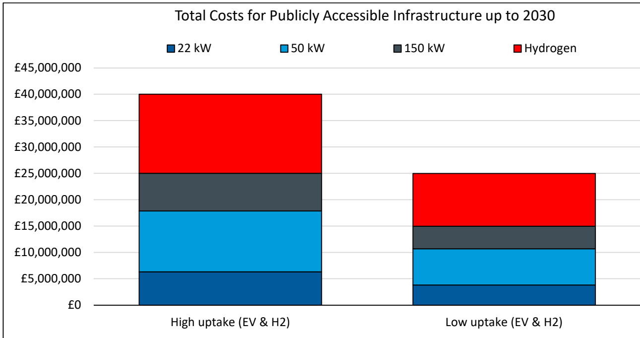
Figure 12-13 - Total public infrastructure costs up to 2030, Western Gateway
