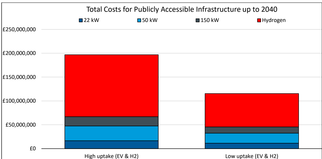
Figure 12-18 - Total public infrastructure costs up to 2040, Peninsula Transport
